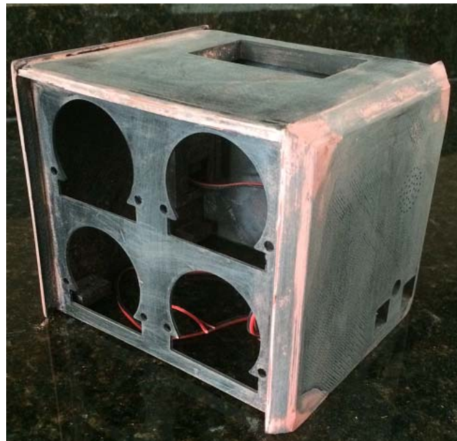
Figure 5.74 – Enclosure Preparation 2
