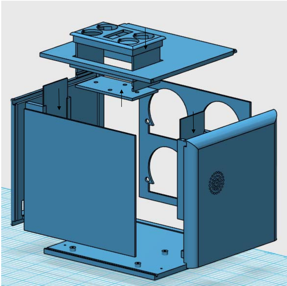
Figure 4.14 – Assembly View 4
