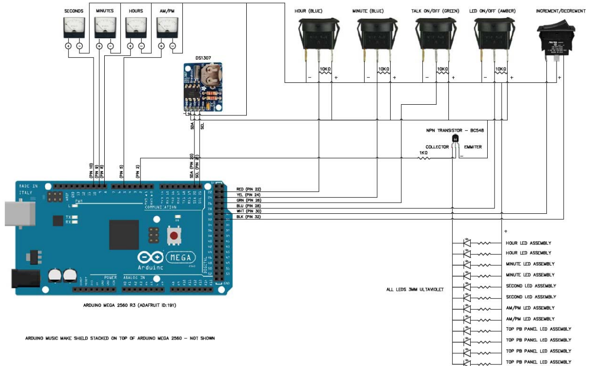
Figure 5.191 – Wiring Diagram
